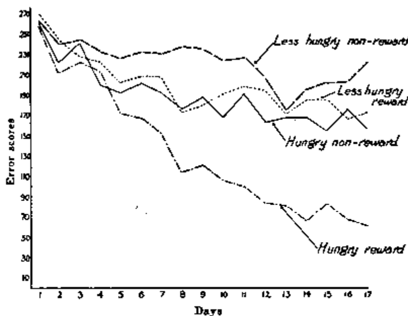
Error curves for four groups, 36 rats.
